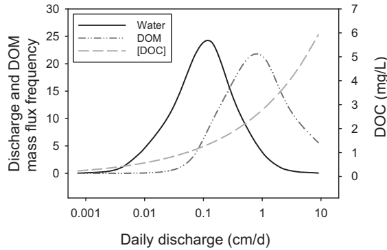
FIG. 2. Discharge frequency and the contribution of events to dissolved organic carbon (DOC) export for a representative first-order New England watershed. The discharge frequency (shown on a log scale) was calculated for 15 discharge bins from three small United States Geological Survey (USGS) watersheds (USGS sites 01093800, 01105600, 0106400) spanning the latitude of New England. The figure depicts a smoothed curve of these bins. DOC concentration was estimated from these discharge data using equations from Raymond and Saiers (2010) to calculate DOC according to Eqs 10–12, and is shown as the dashed line. According to this figure, the peak in daily discharge frequency of dissolved organic matter (DOM) is at a daily discharge of \sim 0.15 cm/d. The DOC flux frequency peaks at a discharge closer to 0.8 cm/d, or where the DOC concentration curve crosses the flow-frequency curve. This is known as the effective discharge for DOC.
