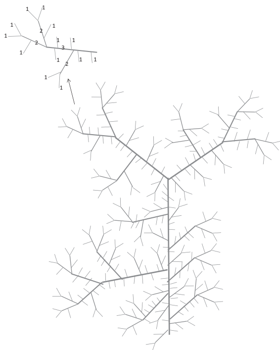
FIG. 1. A visual representation of the first five orders of the representative eighth-order New England (USA) watershed used in the model.
