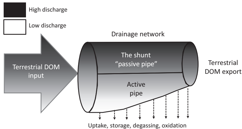
FIG. 4. A conceptual figure of the PSC modified from Cole et al. (2007). According to this figure, terrestrial DOC input is dominated by high-discharge events, encapsulating the high effective discharge for DOC export from headwater streams. Much of the DOC from these high-discharge events enters a passive pipe and is transported conservatively, or shunted through the drainage network and exported. DOC that enters the watershed at lower to moderate discharge events enters the active pipe, where it may be processed and is not exported.
