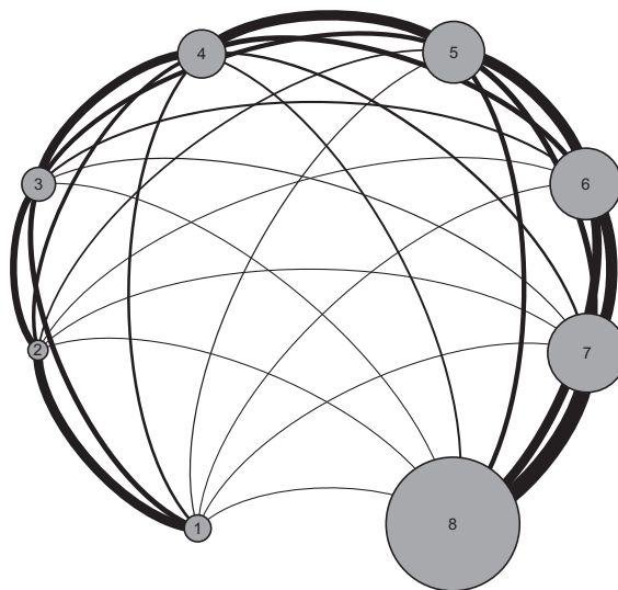
FIG. 3. A network graph for predicted annual uptake of terrestrial DOC among stream orders for a hypothetical large forested watershed using the pulse-shunt concept (PSC) modeling framework and assumptions outlined in this study. The amount of utilized DOC in each stream order is depicted by the size of the circle. The amount of this utilized DOC that was added from each preceding stream order is depicted by the size of the connected lines. In this example, the PSC predicts an annual DOC input from the terrestrial landscape of 1.8 \text{ g} \cdot \text{m}^{-2} \cdot \text{yr}^{-1} , and total drainage network uptake (the sum of all lines) of 1.3 \text{ g} \cdot \text{m}^{-2} \cdot \text{yr}^{-1} . For stream order 8, 46% of the utilized organic carbon was from stream order 7 ( \text{SO}_7 ), 27% from \text{SO}_6 , 14% from \text{SO}_5 , 7% from \text{SO}_4 , 3.3% from \text{SO}_3 , 1.5% from \text{SO}_2 , and 1.2% from \text{SO}_1 .
